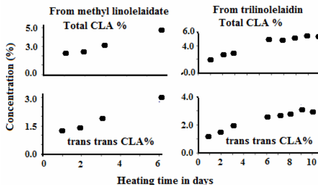
Fig. 4. The concentration of total CLAs and the trans, trans CLAs.
