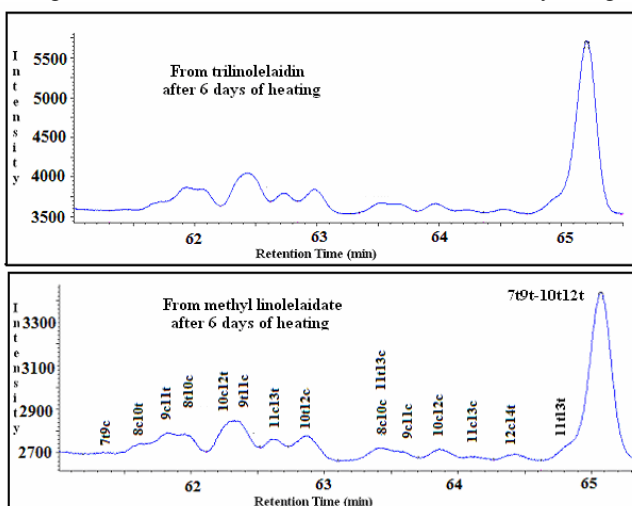
Fig. 3. The parts of the chromatograms indicating the area where CLAs are eluted
