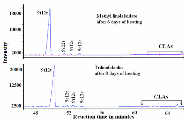
Fig.1. The gas chromatograms of the FAME of the heat treated trilinoelaidin and methyl linoleaidate.
