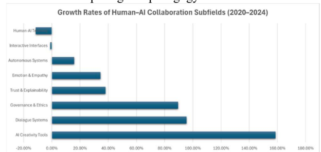
Fig. 3. Subfield compound growth rates from 2020 to 2024.
