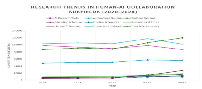
Fig. 1. Yearly publication trends of nine subfields of Human–AI Collaboration from 2020 to 2024.
