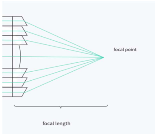
Fig. 4. Fresnel diffraction lens imaging optical path.
