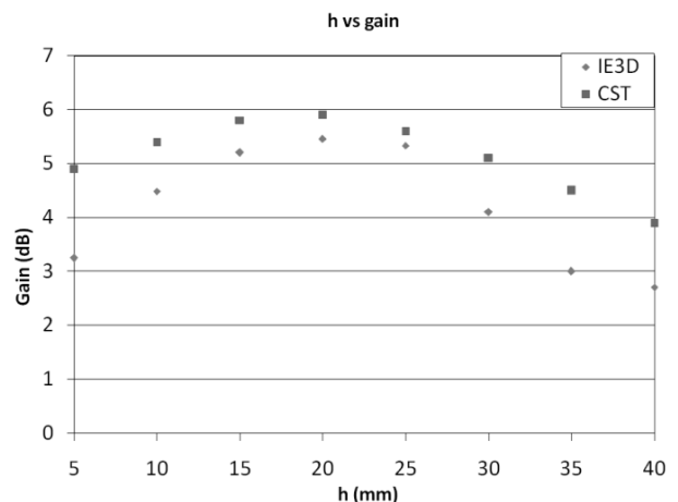
Fig. 5 Variation of proposed antenna's gain with ' h '
