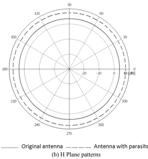
Fig. 3 Radiation patterns comparison for conventional antenna and antenna with parasitic (for d=20 ); CST results
