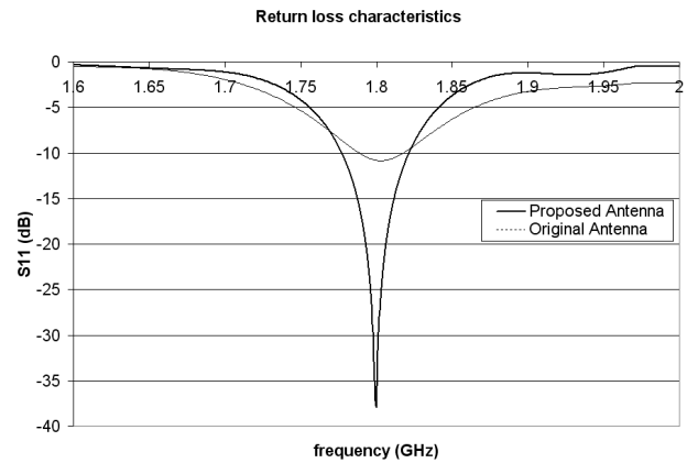
Fig. 2 Return loss vs frequency characteristics comparison (CST simulation) for h=20 mm
