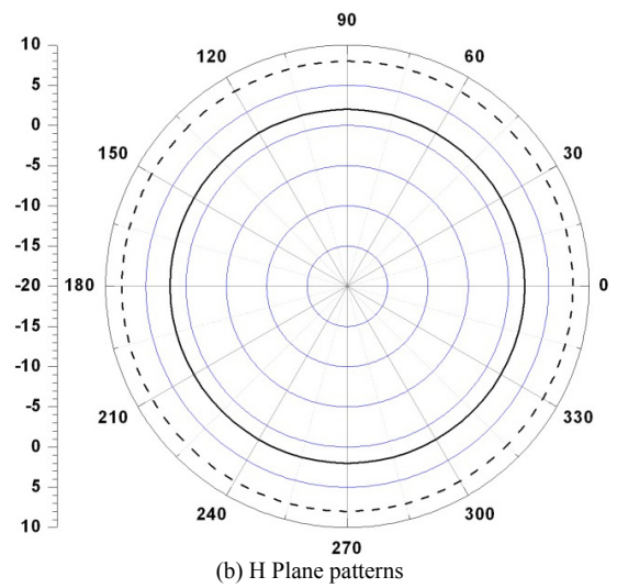
Fig. 4 Radiation patterns comparison for conventional antenna and antenna with parasitic (for h=20 ); IE3D results
