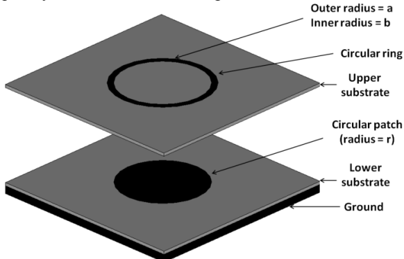
Figure 1 Geometry of proposed antenna
