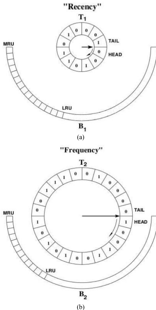
Fig. 2. Working of Clock with Adaptive Replacement
