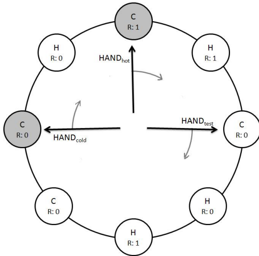
Fig. 1. Working of CLOCK-Pro
