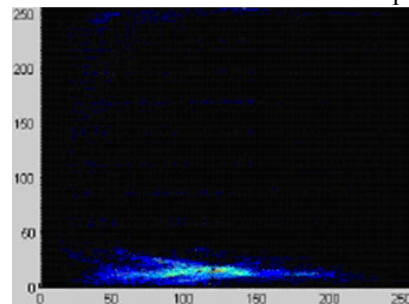
Fig. 1 The histogram of skin color in HS two-dimensional space (adapted from [5]).
