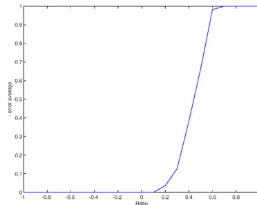
Fig. 11 The curve for average error based on R coefficient for the video images bank.
